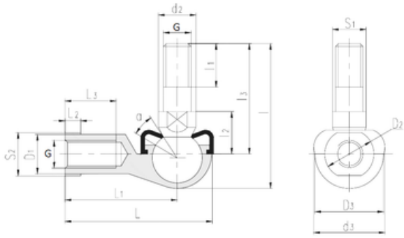
Bearing No. SQ18-RS
