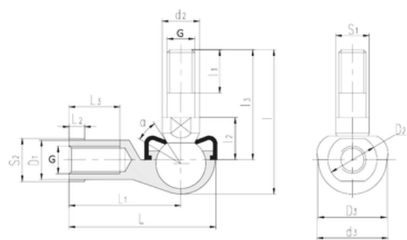
Bearing No. SQ22-RS
