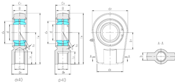
Bearing No. SIRN40ES
