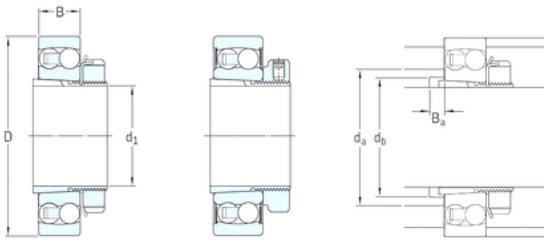
Open bearing on a standard sleeve
