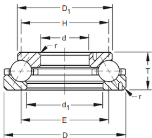
Bearing No. 120TVL700
