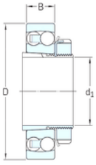
Open bearing on a standard sleeve
