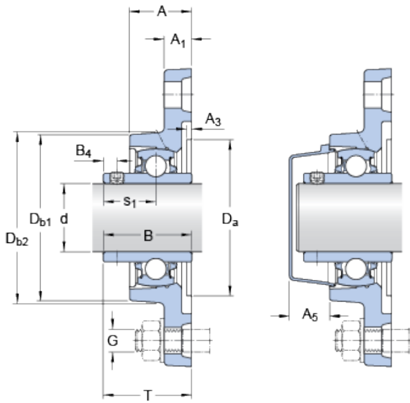
Bearing No. FYTB 1.1/2 TDW
