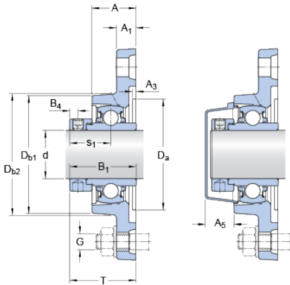
Bearing No. FYTB 1.1/2 WDW
