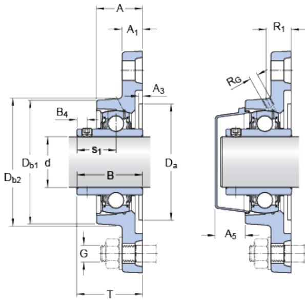
Bearing No. FYTB 1.1/4 TF
