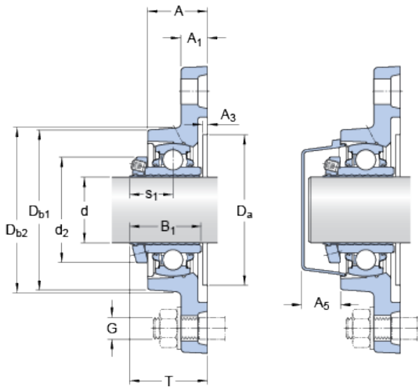
Bearing No. FYTB 1.3/16 LDW
