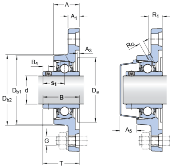
Bearing No. FYTB 25 TF
