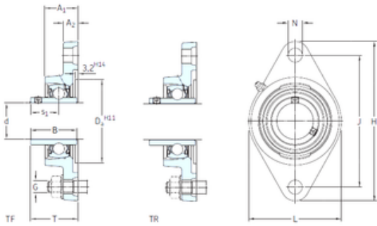
Bearing No. FYTB 25 WF
