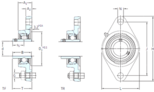
Bearing No. FYTB 40 TR
