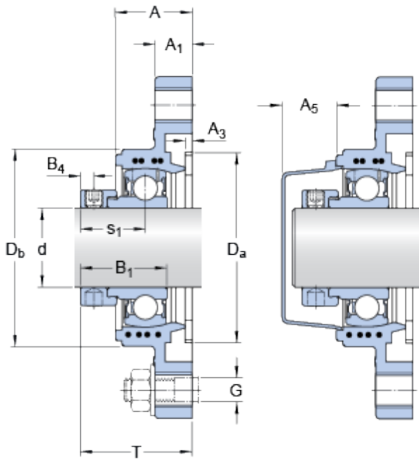
Bearing No. FYTBK 20 FE
