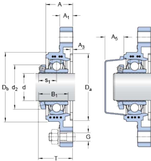
Bearing No. FYTBK 30 LEF
