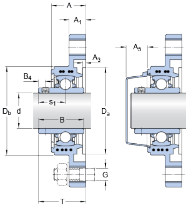
Bearing No. FYTBK 35 TD
