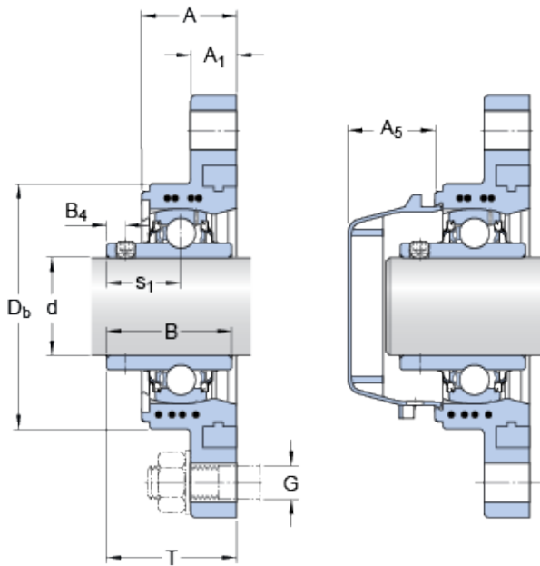
Bearing No. FYTWK 1.3/8 YTA
