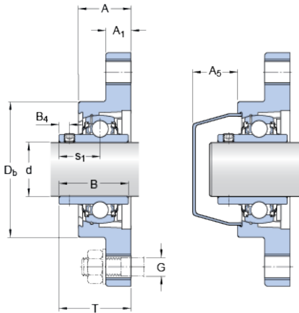
Bearing No. FYTWK 40 LTHR
