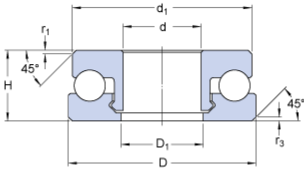
Bearing No. 51201 V/HR11Q1
