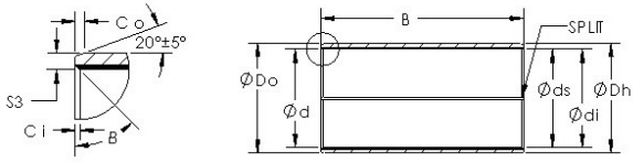
Bearing No. AST850BM 13580
