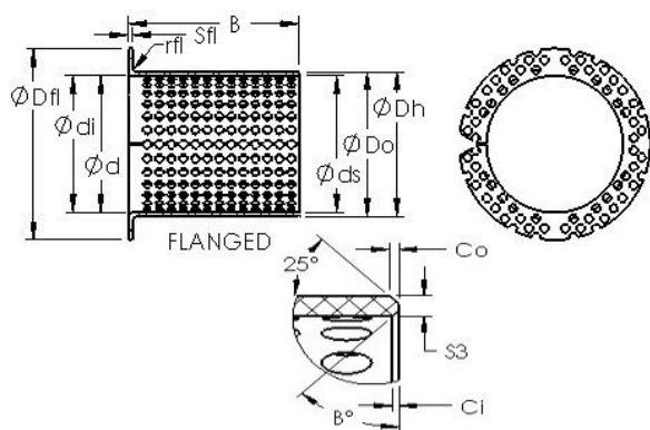
Bearing No. ASTT90 F12060
