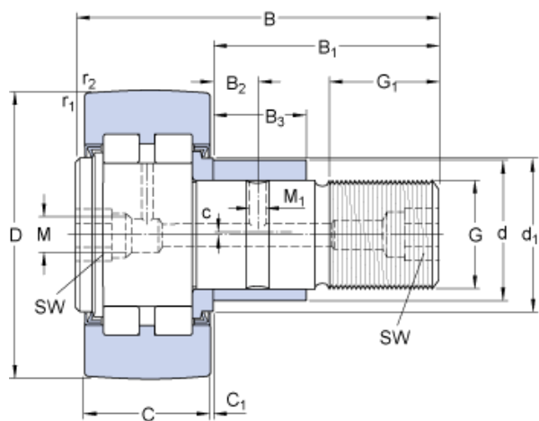
Bearing No. PWKRE 47.2RS
