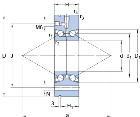
Bearing No. BEAM 012055-2RZ
