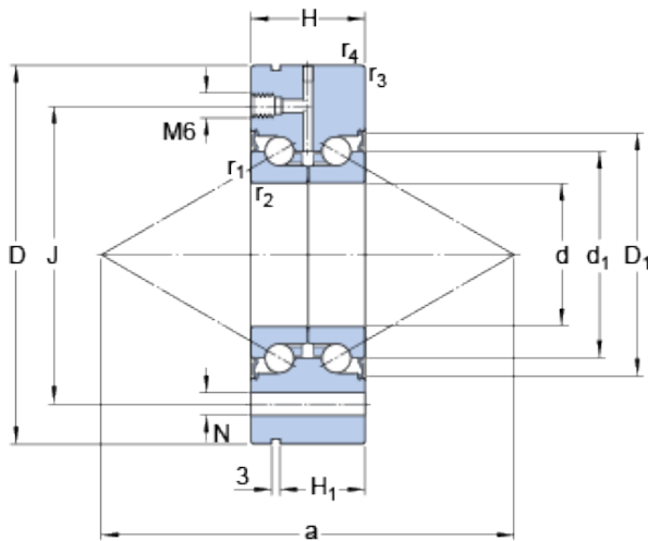
Bearing No. BEAM 017062-2RS/PE
