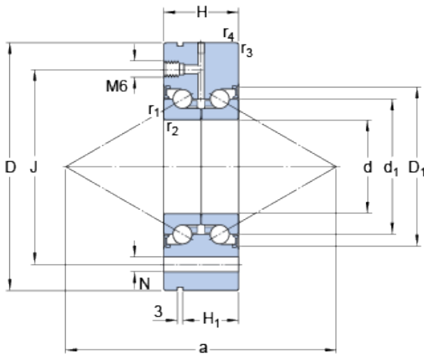
Bearing No. BEAM 020068-2RZ/PE
