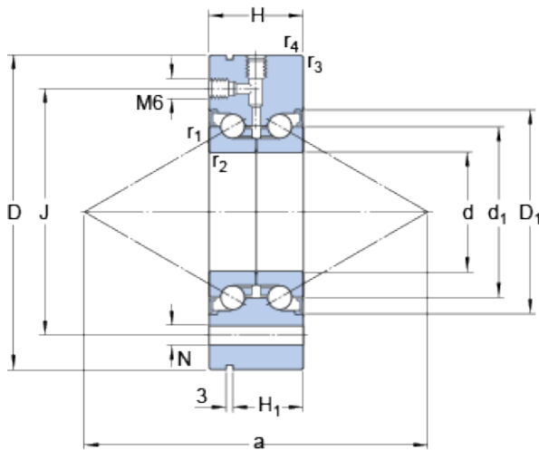
Bearing No. BEAM 030080-2RZ
