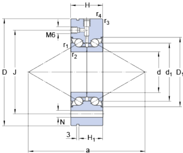
Bearing No. BEAM 030100-2RS
