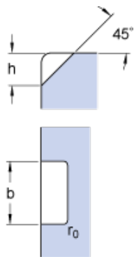
Bearing No. QJ 212 N2MA
