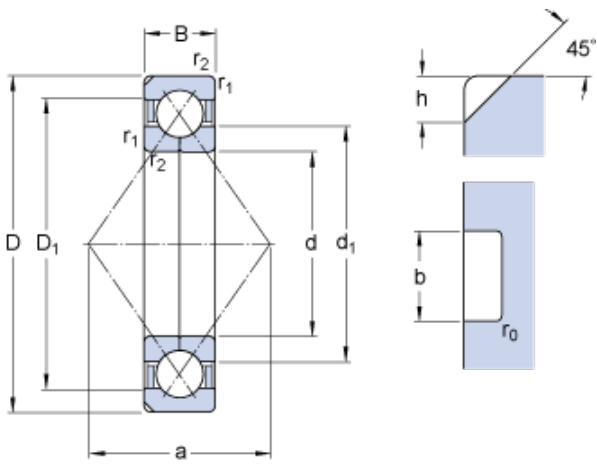
Bearing No. QJ 1260 N2MA
