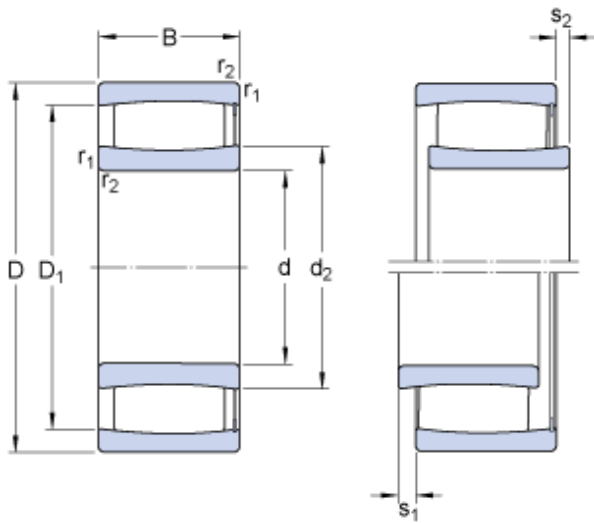
Bearing No. C 2212 V
