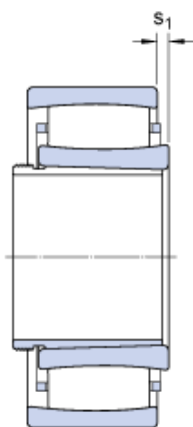
Bearing No. C 2224 K + AHX 3124
