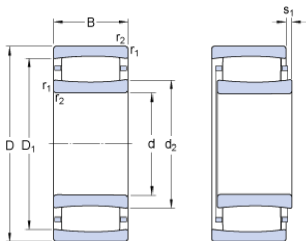
Bearing No. C 2316
