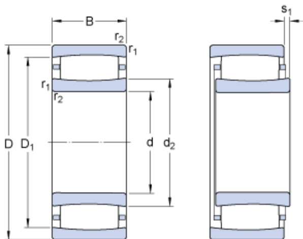
Bearing No. C 30/850 MB
