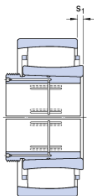
Bearing No. C 3048 K + AOH 3048
