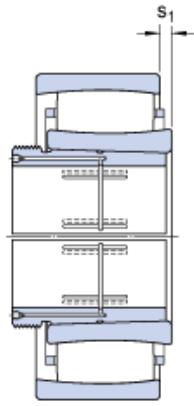
Bearing No. C 3052 K + AOH 3052
