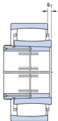
Bearing No. C 3088 KMB + AOHX 3088 G
