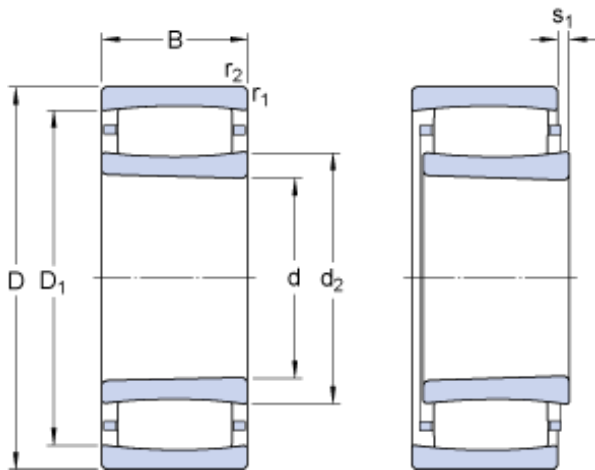
Bearing No. C 31/850 KMB
