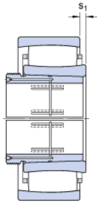
Bearing No. C 3192 KM + AOHX 3192 G
