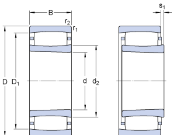
Bearing No. C 39/750 KM
