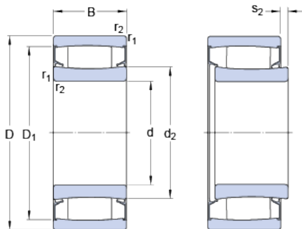
Bearing No. C 4026-2CS5V/GEM9
