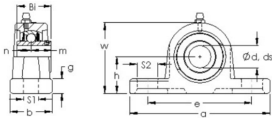
Bearing No. UCP 212
