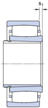
Bearing No. C 4134 K30V + AH 24134
