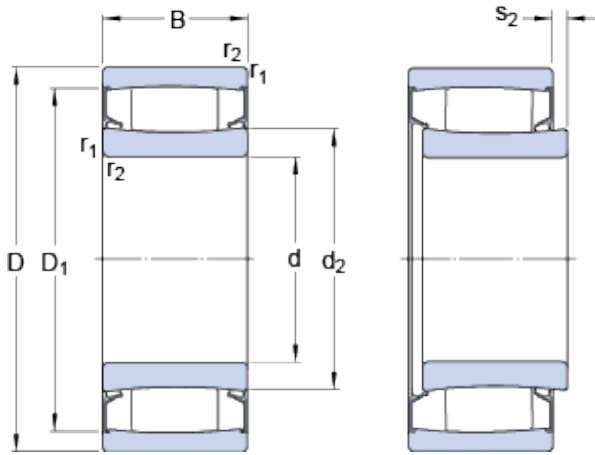
Bearing No. C 4136-2CS5V/GEM9
