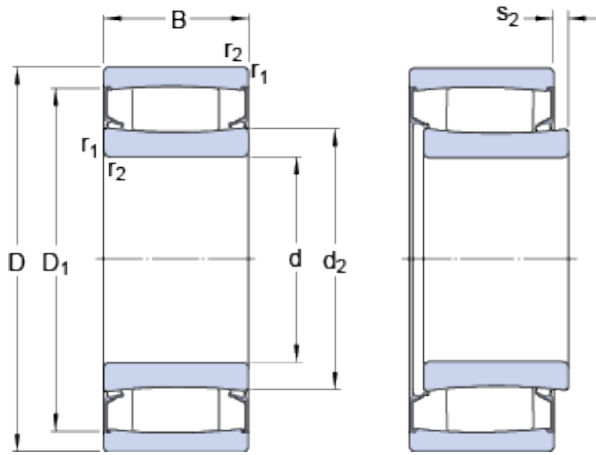
Bearing No. C 4138-2CS5V/GEM9
