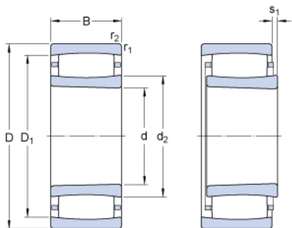
Bearing No. C 49/750 K30MB1
