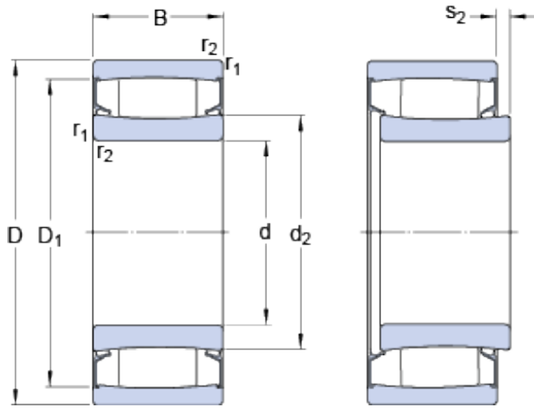
Bearing No. C 6910-2CS5V/GEM9
