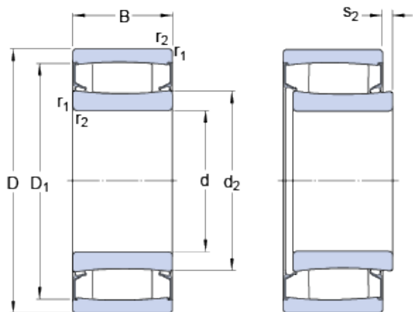
Bearing No. C 6915-2CS5V/GEM9
