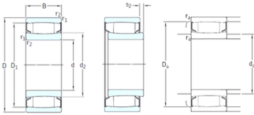
Bearing No. C4124-2CS5V/GEM9
