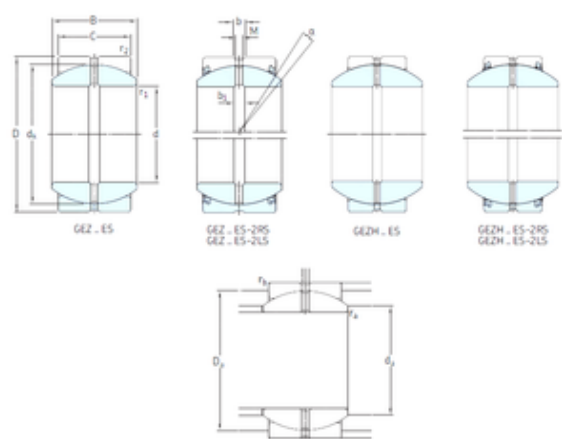
Bearing No. GEZH200ES-2RS
