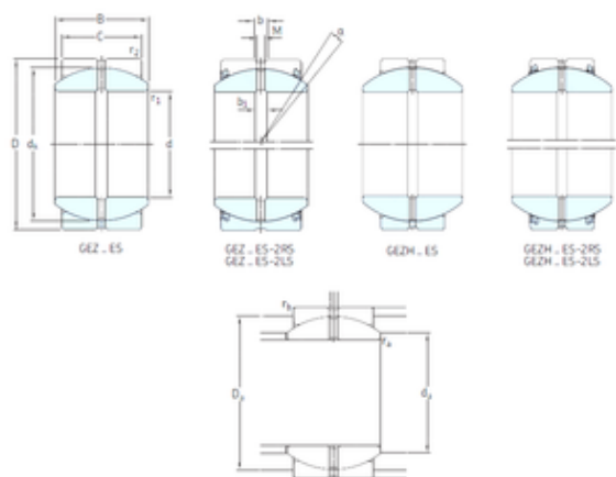
Bearing No. GEZH400ES-2LS
